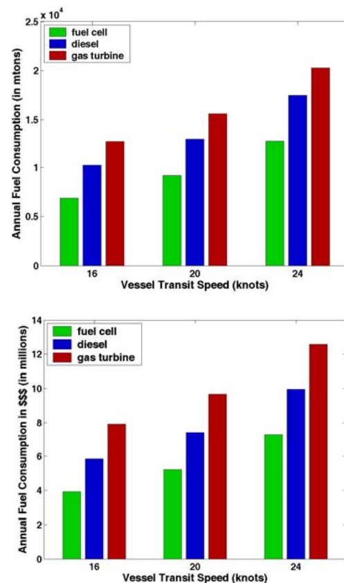
Figure 11: Annual fuel consumptions for three different power plants.
