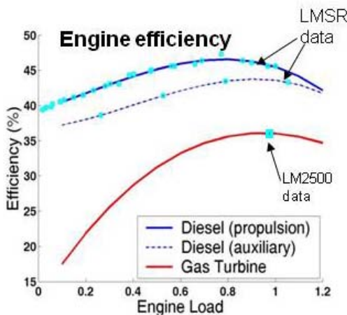
Figure 9: Power plant efficiencies used in fuel consumption calculation.
