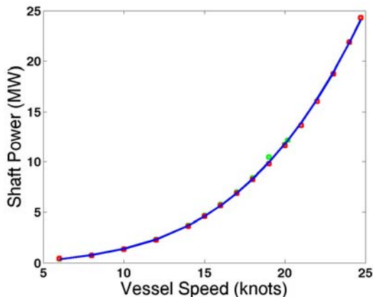
Figure 2: Propulsion power demand as a function of vessel speed.
