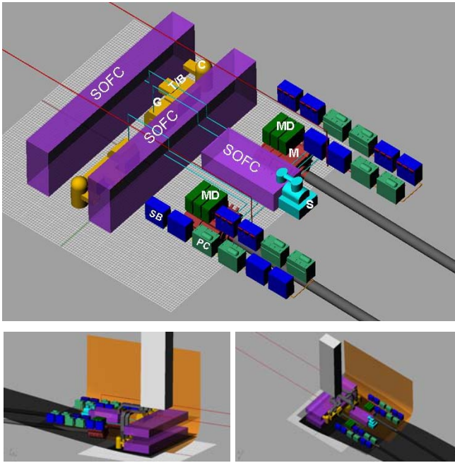
Figure 15: Machinery arrangement of configuration B (refer to Figure 14 for the legends).
