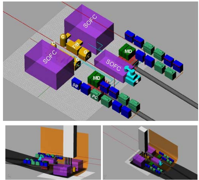
Figure 14: Machinery arrangement of configuration A.
