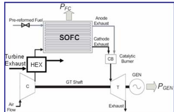
Figure 5: Schematic of the hybrid SOFC-GT system.
