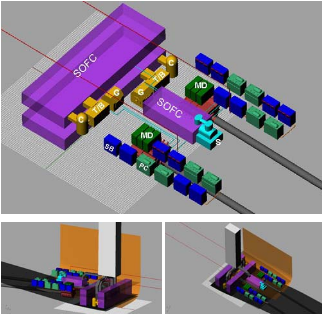
Figure 16: Machinery arrangement of configuration C (refer to Figure 14 for the legends).
