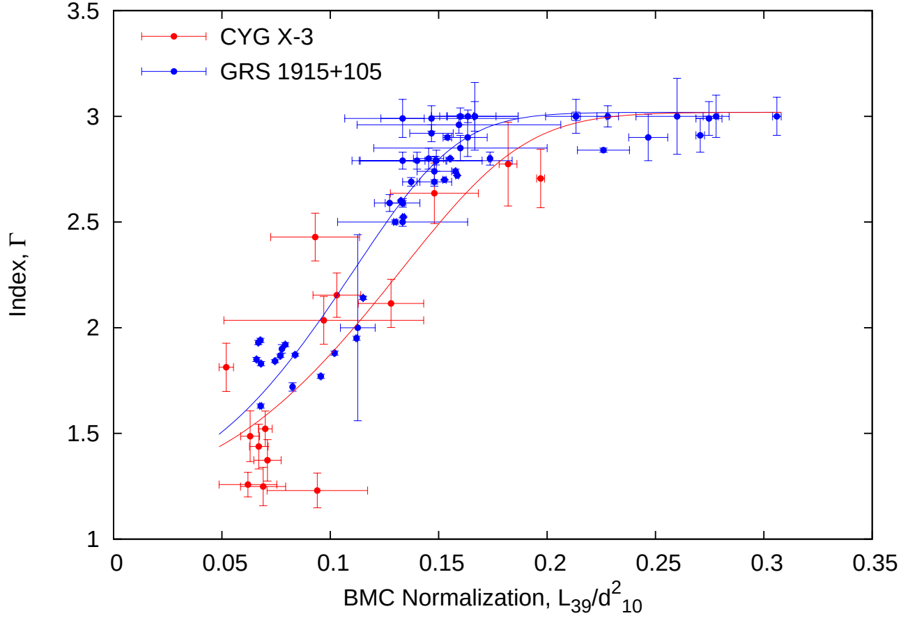
Fig. 4.— Spectral index \Gamma –normalization diagram for Cyg X-3 (red points) in comparison to the our reference source, GRS 1915+105 (blue points). The normalization term, derived from our model, scales with the mass-accretion rate. The smooth curves represent the best fits of the functional form of equation 1 to the respective datasets. The derived scaling parameters, as discussed in section 3.3, lead to an estimated mass of for the compact object in Cyg X-3 consistent with a black hole.
