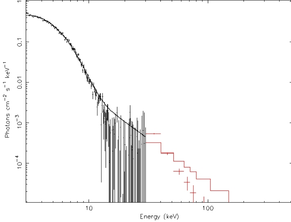
Fig. 2.— Example of an extreme soft state case, not well suited for our mass-estimation analysis. The hard-powerlaw index parameter is clearly poorly constrained by the data for this spectral-state configuration of the source. The corresponding data would lead to a point in the far left-hand side of Figure 1.
