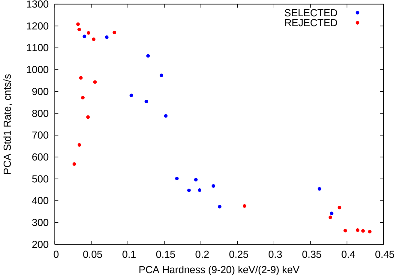
Fig. 1.— Hardness-intensity plot for the RXTE data considered. The data which were used in our mass-determination procedure are plotted as the blue points, while the cases where our model did not fit the data satisfactorily are red. Note that the red points are generally at the extremes in terms of spectral state configuration of the binary.
