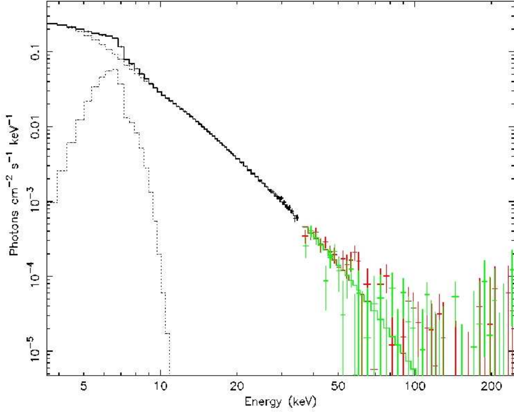
Fig. 3.— Example of one of our satisfactory model fits to the data as described in section 2. Here the spectral index is hard, \sim 1.5 , well below the saturation level but within the expected range. In this case the model fits the data at an acceptable level and the mass-estimation parameters are well defined.
