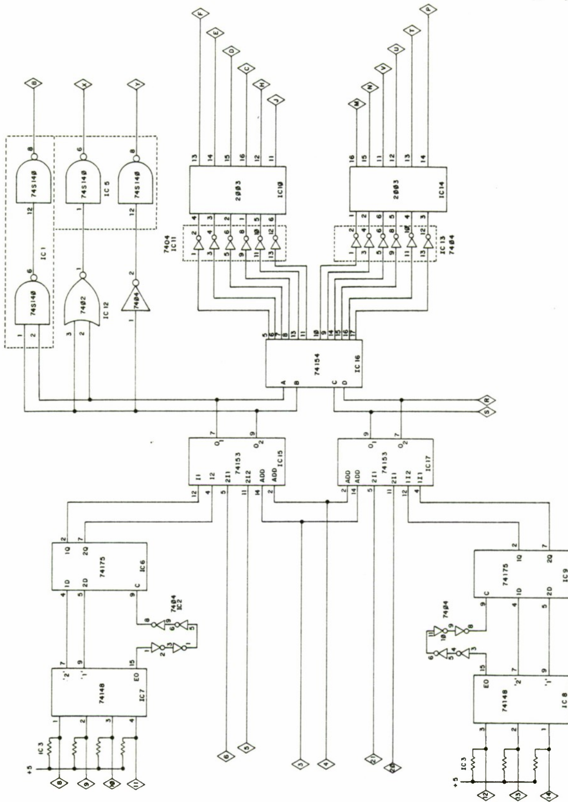
Figure 6 - Control Board PLL-12
