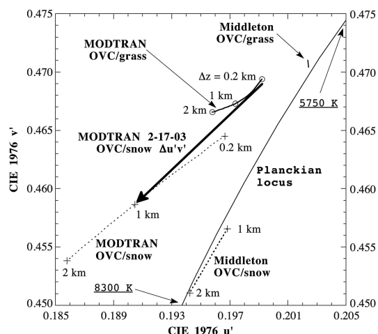
Fig. 18. MODTRAN simulations of stratus overcast u' , v' chromaticities at the zenith as functions of cloud \Delta z and the underlying surface’s spectral reflectance r_\lambda . The thick arrow indicates MODTRAN’s prediction of the chromaticity shift caused by changing the surface from grass to snow for Fig. 19’s observed changes in cloud \Delta z . For historical purposes, we also include overcast chromaticities simulated by Middleton. 4
