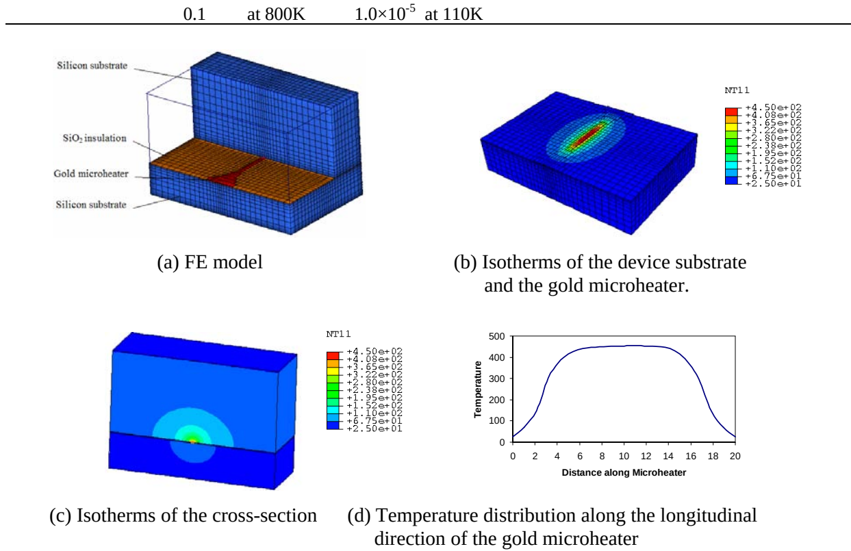
Fig.3 Line-shape FE modeling of localized heating
