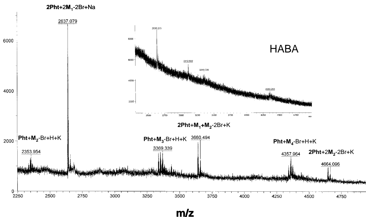
Figure 9. MALDI mass spectra of (Cp) styryl POSS in 4,4'-dihydroxyoctofluoroazobenzene. Inset shows spectrum in HABA matrix.
