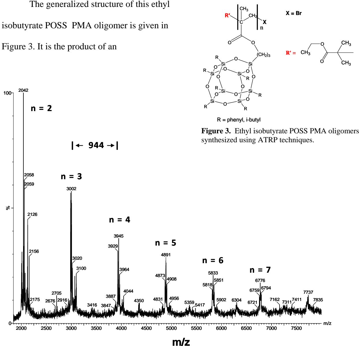
Figure 4. ESI mass spectrum of \text{CH}_3\text{CH}_2\text{OOC}-\text{C}(\text{CH}_3)_2-[(i\text{-butyl})_7\text{T}_7\text{propylmethacrylate}]_n . Most intense peaks are assigned to sodiated and potassiated parent species, the terminal Br being replaced with OH.
