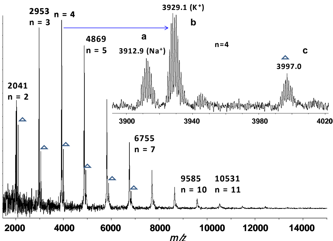
Figure 5. Ethyl isobutyrate Isobutyl POSS PMA MALDI mass spectrum using 4,4'-dihydroxyoctoflyoroazobenzene matrix. Typical series (a-c) shown in expansion in region of m/z = 3900 - 4020
