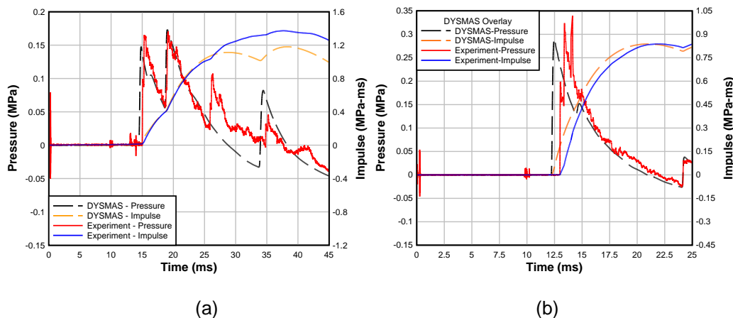
Figure 2 Overlay of reflective pressure gauges at the (a) base of the structure and (b) at mid-height
