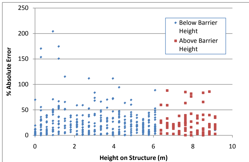
Figure 6 Bias of peak pressure errors towards heights on the structure face below the height of the blast wall
