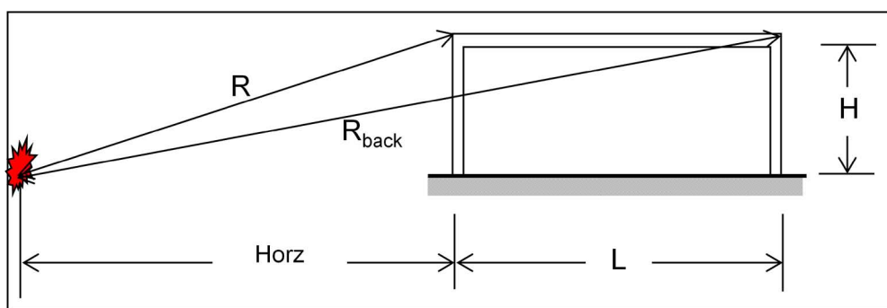
Figure 10 Factors for predicting blast loading to roofs
