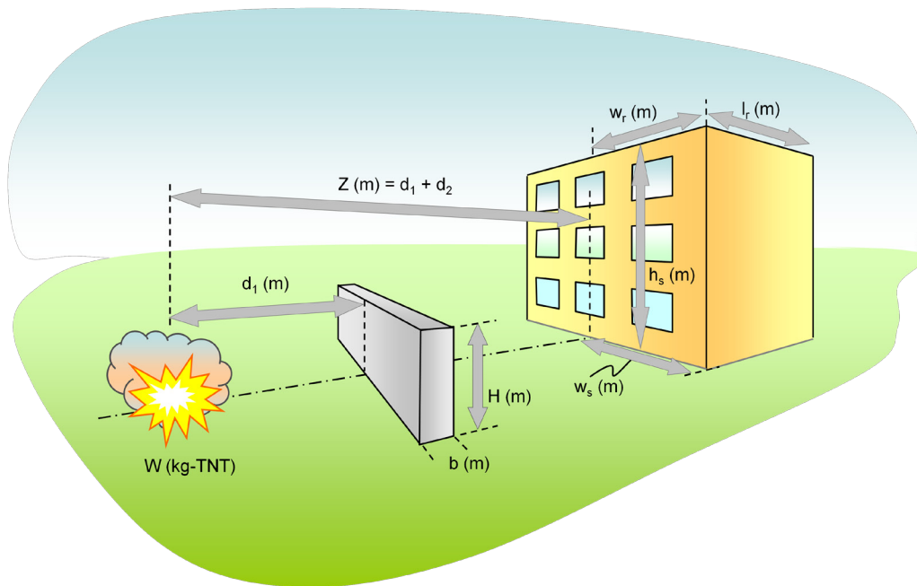
Figure 1 Blast barrier wall configuration
