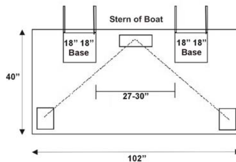
Figure 5. Schematic representation of the mounting positions for the cable take-up and the tow point pads.
