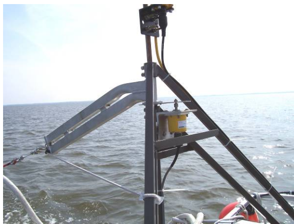
Figure 2-9. The tow point, mounted at the rear of the boat supports the master GPS antenna located on the mast. The digital encoder (yellow) measures the angle of the tow cable relative to the boat heading. The weak link cable is located between the shackles at the end of the tow arm.
