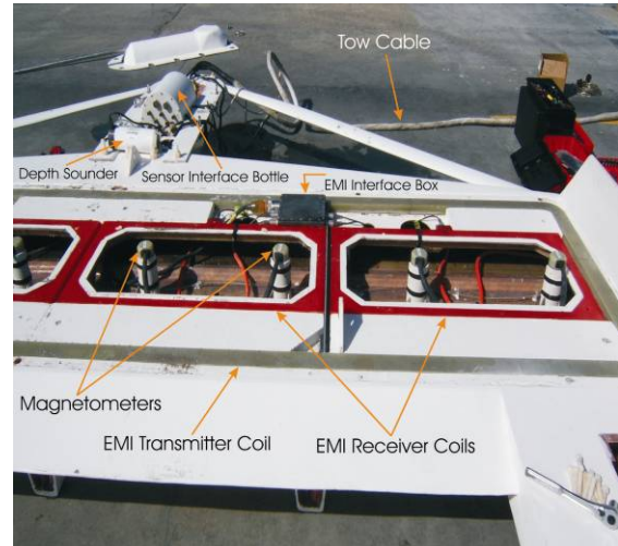
Figure 2-5. The marine sensor platform is shown with the hatch covers removed.
