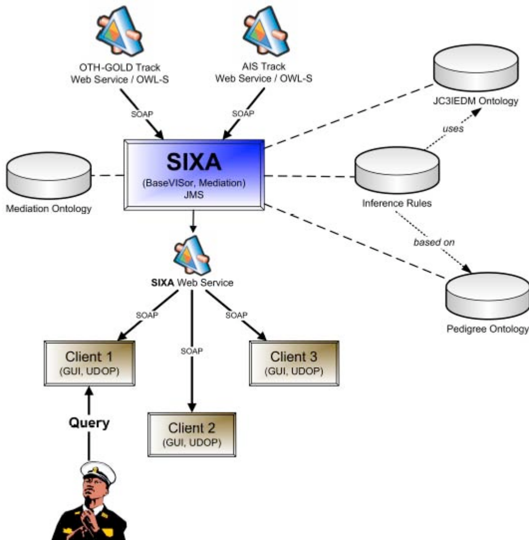
Figure 1. The initial SIXA Architecture
