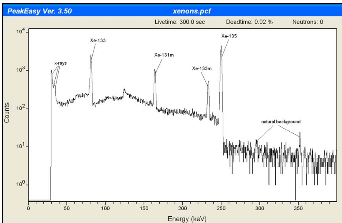
Figure 1. Gamma-ray Signatures of Four Radioactive Isotopes or Isomers of Xenon
