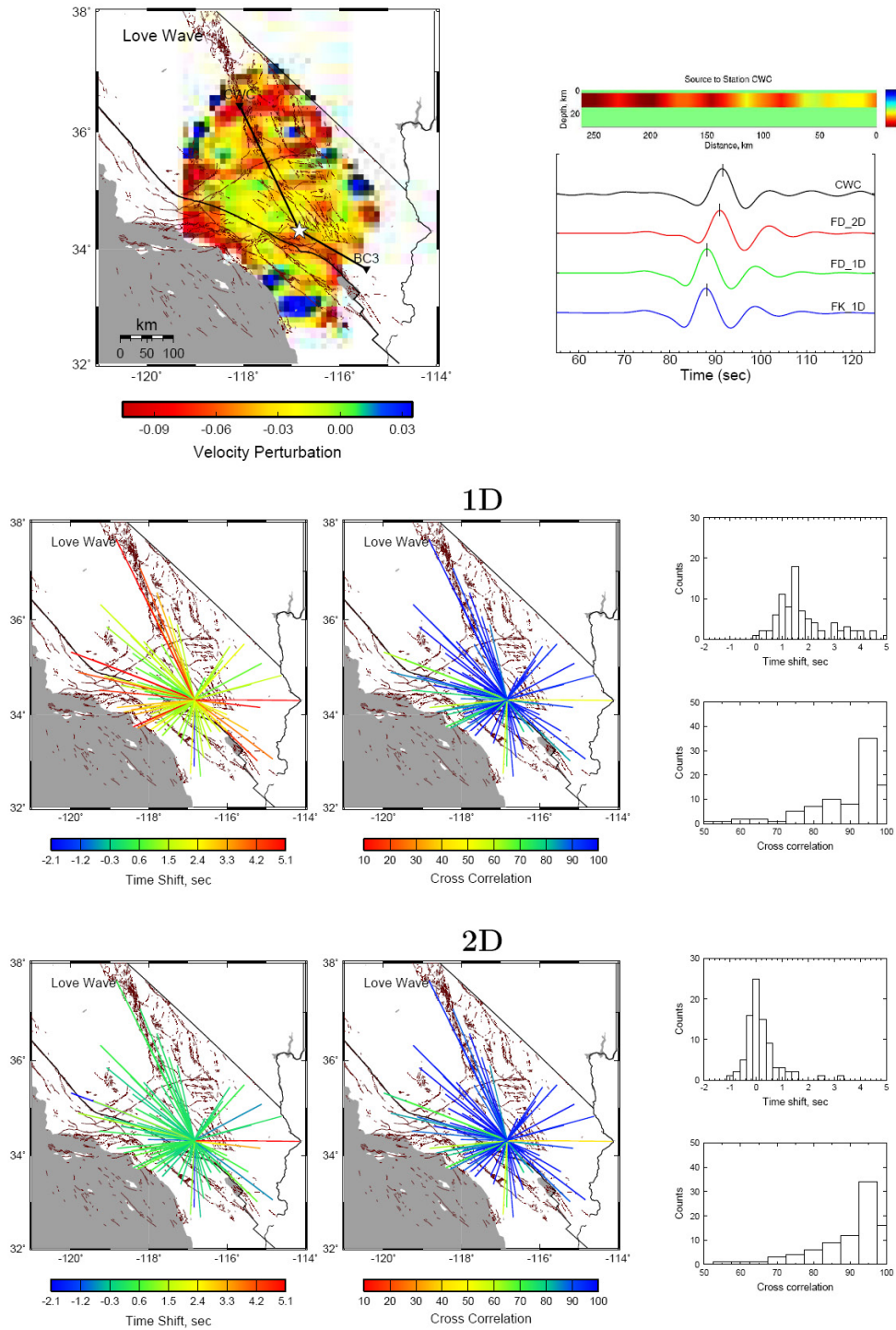
Figure 3. The top panel displays the Love wave phase velocity perturbation in southern California with a selected source (star)-receiver (triangle) path, along which the 2D cross section is shown and the synthetics are compared against the data on the right. The lower panel summarizes the comparison between 1D and 2D synthetics against the observed Love waves for a Big Bear event.
