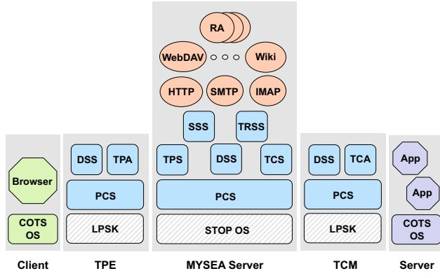
Figure 2: MYSEA Software Architecture
