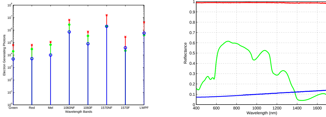
Figure 4.18: (Left) The number of electron-forming photons hitting the focal plane array of each camera with three different targets. The red × represents the white Spectralon ® panel, green * represents skin, and blue o represents the gray Spectralon ® panel. The labels on the x axis of red and green correspond the color channels for Camera 1 ; Mel corresponds to Camera 2 ; 1060NF and 1570NF correspond to what Camera 3 and Camera 4 see with only their respective mirrors reflecting and transmitting; 1060F and 1570F correspond to the use of the Semrock bandpass filters on Camera 3 and Camera 4 . Lastly, LWPF corresponds to the use of the Reynard corporation longwave pass filter on Camera 4 . (Right) The measured reflectance of each target shown in the model. Red corresponds to the white panel, green corresponds to skin, and blue corresponds to the gray panel reflectance.
