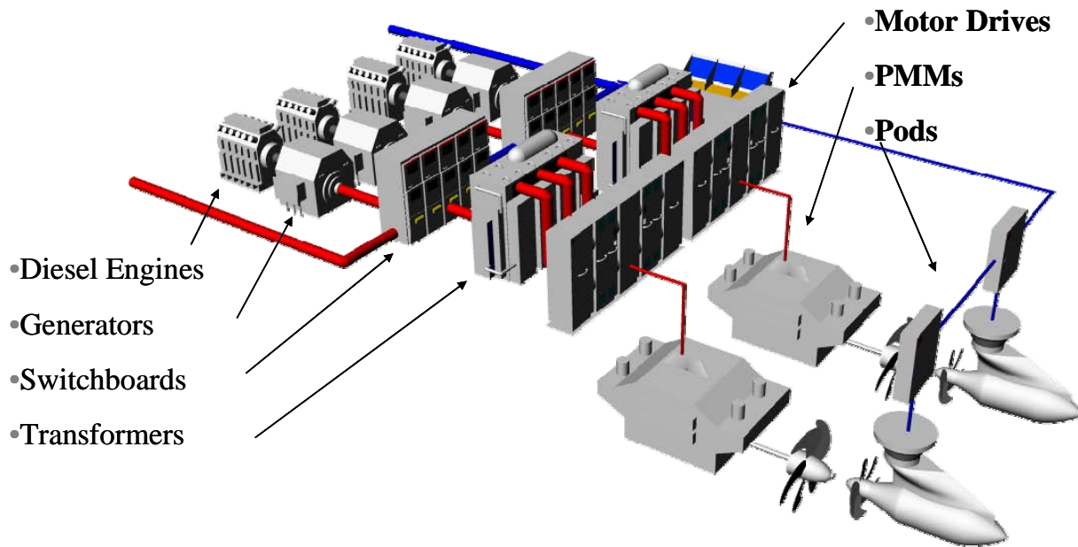
Figure 14. Propulsion Arrangement
