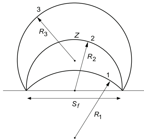
FIGURE 5 Flux-rope scaling law. The arcs schematically represent a rising flux rope.
