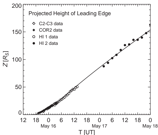
FIGURE 6 Theoretical solution directly compared with SECCHI data. Measured height-time data are represented by various symbols corresponding to different telescopes. The curve is the "best-fit" theoretical solution.
