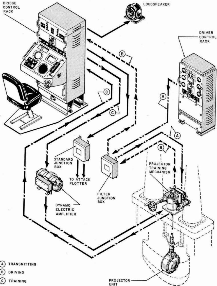
Figure 3. Pictorial diagram of the QGB System (Bureau of Naval Personnel, 1953); reproduced with permission from the Historic Naval Ships Association.
