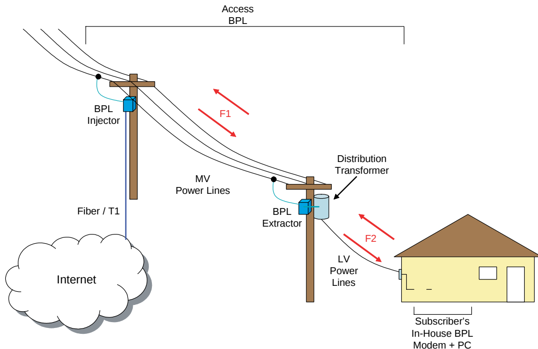
FIGURE 4 Basic BPL system. 1
