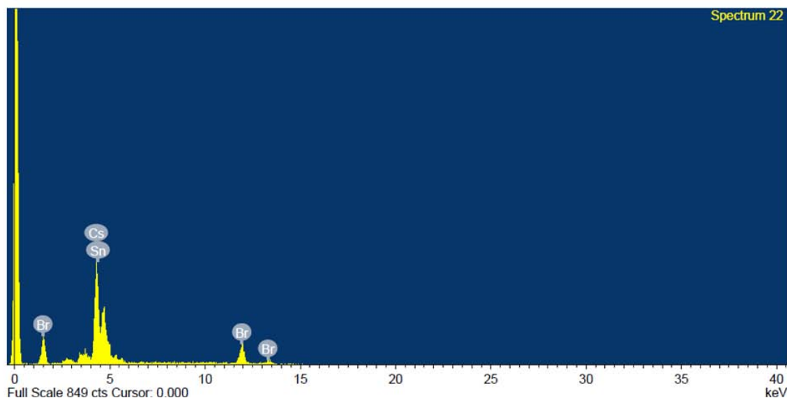
Figure 55. Much like the CL graphs a plot of energy vs. intensity is produced. The elements are identified by their characteristic x-ray fluorescent emissions. This phenomena is the same mechanism by which EXAFS works. The XRF technique is much faster as absorption versus energy dependence is not measured over several energies. An XRF run takes seconds compared to over an hour for an EXAFS run. The Ca is not present in this data sample of CsBr:Sn-1%. The intensity side of the graph is in units of counts. The predominant atoms in the crystal react more often with the x-rays than the impurities. Thus, the Ca signal can be washed out during long runs of data.
