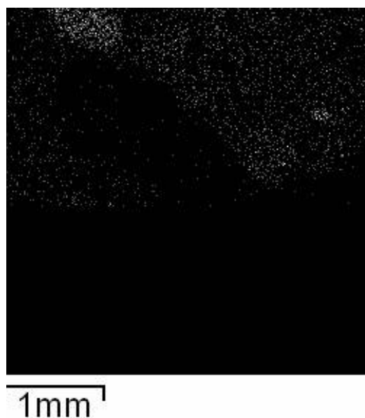
Figure 59. The 1% concentration of Sn is shown evenly distributed throughout the crystal. The response as seen in the image is not as intense as seen for Cs in Figure 57. This is expected as it occurs only 1% of the time in the matrix.
