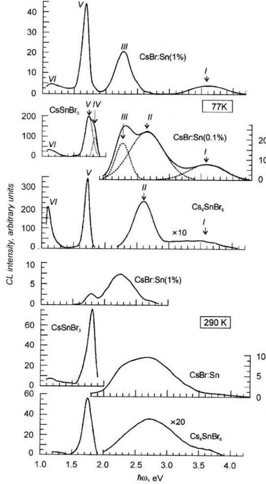
Figure 14. This thesis is aimed at comparing the data at 290K. The equipment setup limited the experiment to room temperature. The figure data shows a response at 2.25-eV for \text{CsBr:Sn-1\%} which is in the yellow to green region. The \text{CsSnBr}_3 shows a peak around 1.75-eV which is around the red region [Savchyn et al., 2007].
