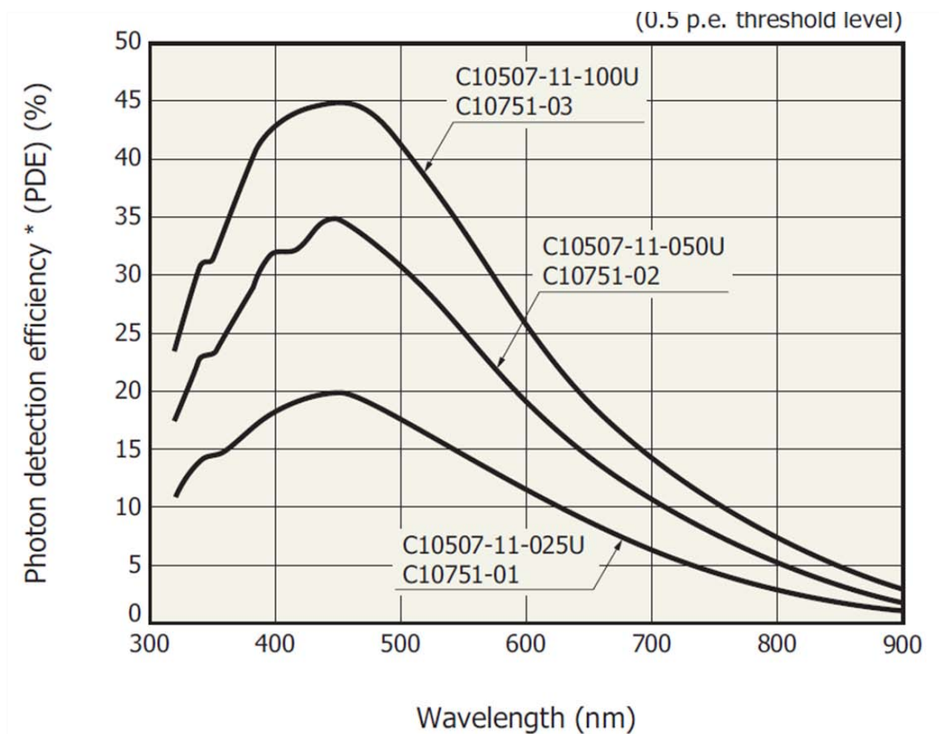
Figure 61. Photon detection efficiency of the Hamamatsu MPPC module as a function of wavelength. The module was used to measure the light yield of different candidate scintillator materials [Division, 2010].
