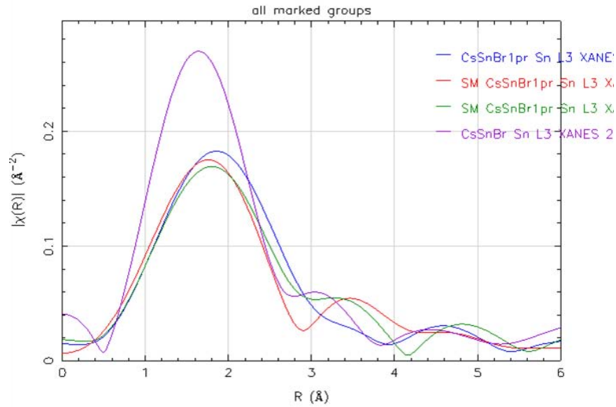
Figure 26. The \text{CsSnBr}_3 , Sn centered, plot is shown in purple. The other plots are Sn centered \text{CsBr:Sn-1\%} . In all cases the distance to the Br peak is shown. There is a little difference in the position of the Br shell between \text{CsSnBr}_3 and \text{CsBr:Sn-1\%} .
