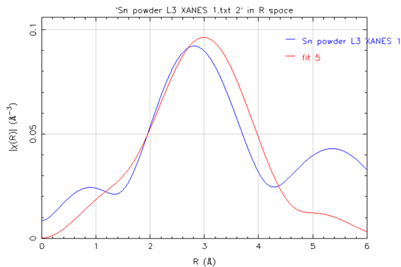
Figure 10. The first shell of Sn in the \beta phase is at 3.01617-Å. The data was processed in Athena and then fit using Artemis. The blue line is the processed data and the red line is the first shell fit using the pre-calculated theoretical paths of the photo electron wave traveling to the first neighbor shell and returning back after reflection.
