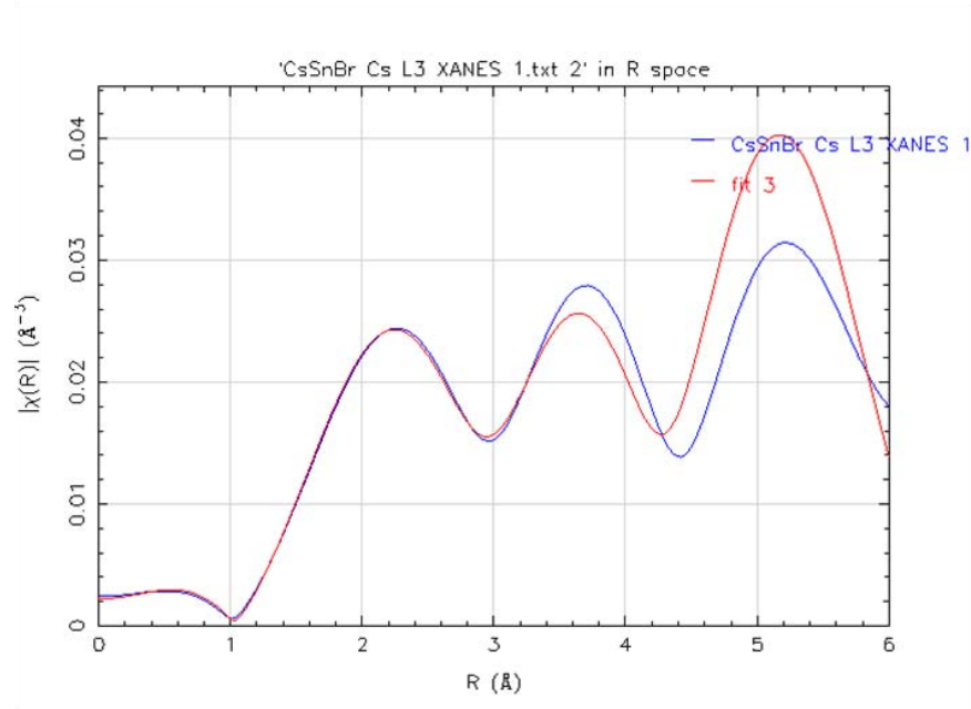
Figure 24. The second peak of this fit is the first shell neighbor of Br atoms at 4.1-Å. Sn second shell neighbors at the third peak at 5.0-Å. The first peak is a half path interference of the Sn shell.
