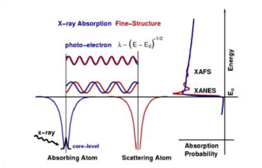
Figure 8. The reflected photoelectron wave representation is shown in the red. The reflecting atom attenuates the photoelectron wave in phase and amplitude. The absorption spectrum shows the constructive and destructive interference of the ideal photoelectron reflection shown in blue. Thus, the spectra following the absorption edge is attenuated causing the XANES and subsequent EXAFS structures at higher energies.
