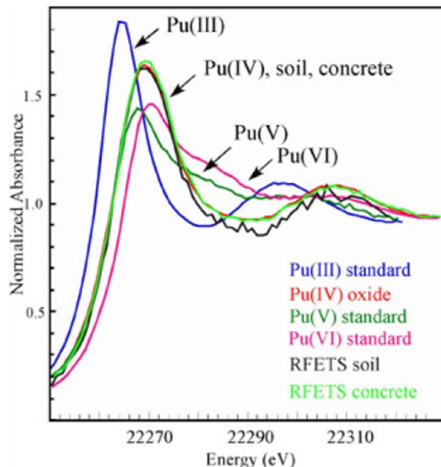
Figure 6. Pu standards in oxidation states of 3+, 4+, 5+ and 6+ were used to identify the Pu pollution in the Rocky Flats area. The identification of the \text{Pu}^{4+} oxidation state aided environmental models in determining the area affected by Pu the leaks [Clark, 2002].
