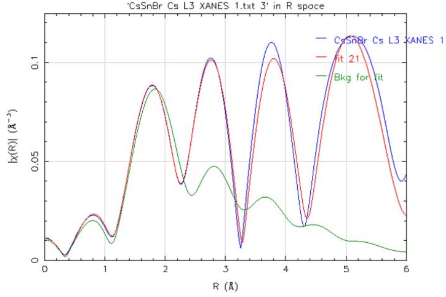
Figure 42. This is a close to good CsSnBr 3 fit using the Fit Background option.
