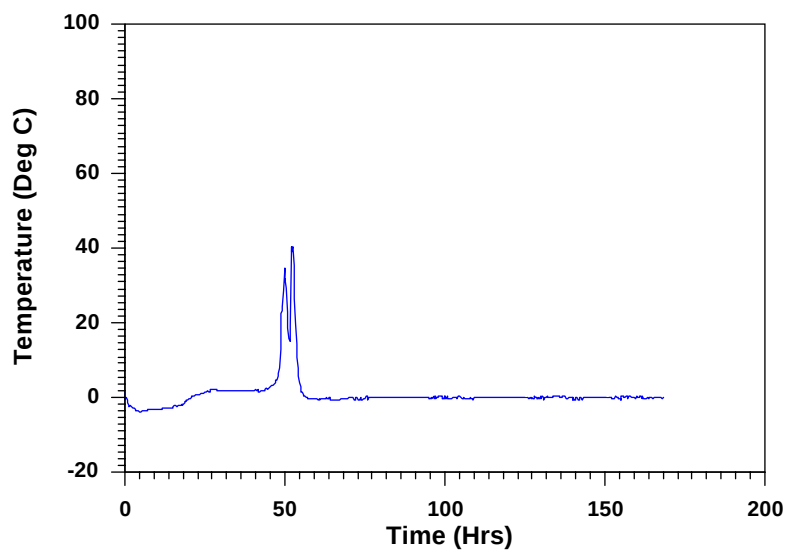
Figure 4 Test #3 Al/ \text{NH}_4\text{NO}_3 /H 2 O
