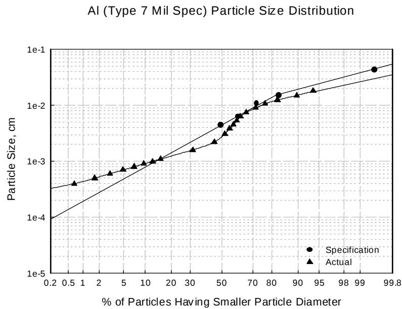
Figure 1 Particle Size Analysis of Aluminum Powder Meeting Mil-A-512A Type III Group F, Class 7
