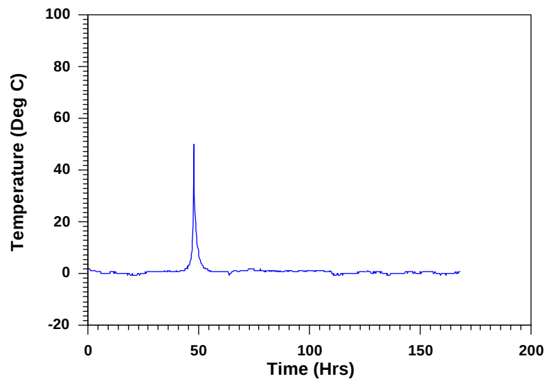
Figure 8 Test # 4 80/20 Al/TNT pH 7.0
