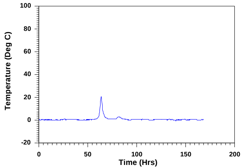
Figure 2 Test #1 Al/Water
