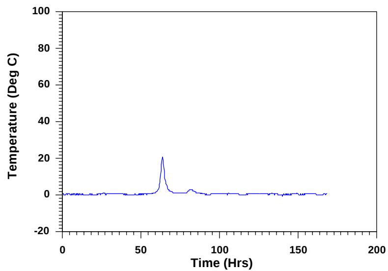
Figure 13 Test #7 Al/Water
