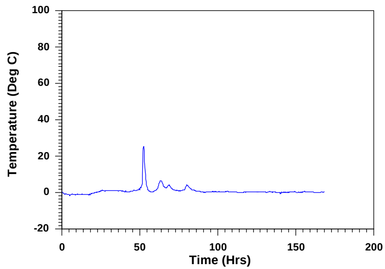
Figure 11 Test #5 Al/Water
