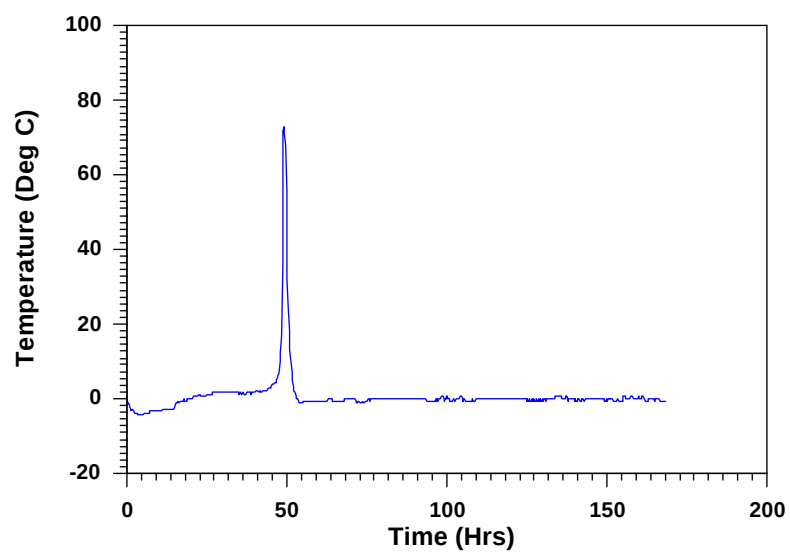
Figure 12 Test #6 Al/Water
