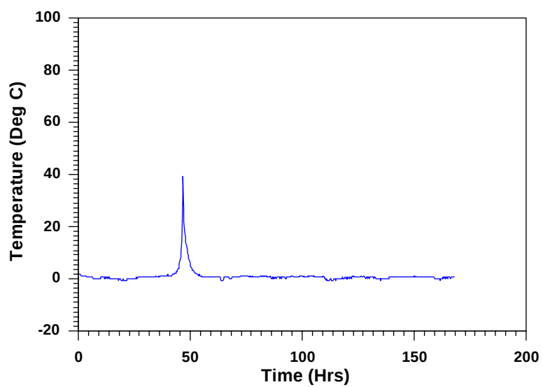
Figure 7 Test # 4 80/20 Al/TNT pH 6.0
