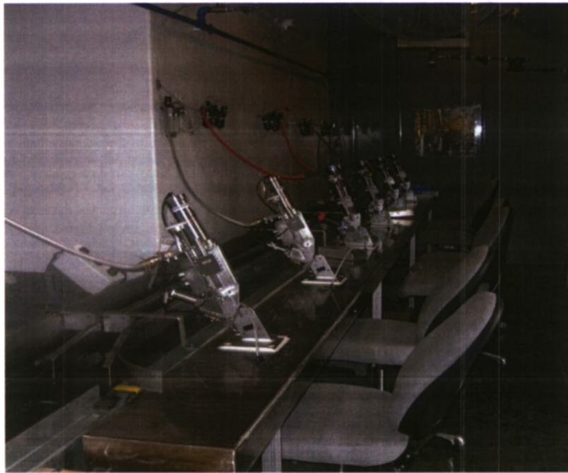
Figure 2 Tipper tie operation with two additional tipper tie machines installed
