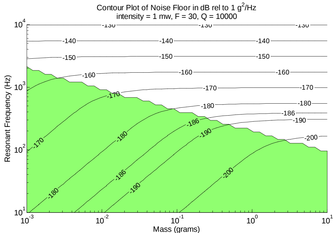
Figure 2. Contours of constant noise floor as a function of the key design parameters, resonant frequency and mass. The target level for the broadband white noise is -186 \text{ dB/Hz} , or 0.5 \text{ ng/Hz}^{1/2} . Within the shaded region, the device is limited by thermal noise. Outside of this region, the limit is photodiode shot noise.
