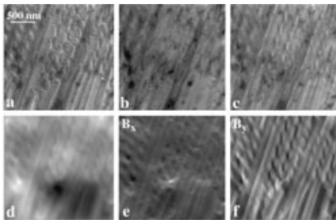
Fig. 4. Similar set of images as in Fig. 1, taken at 300 kV and 118 K. The martensite plates are clearly visible. Two different domain geometries are observed, as discussed in the text.
