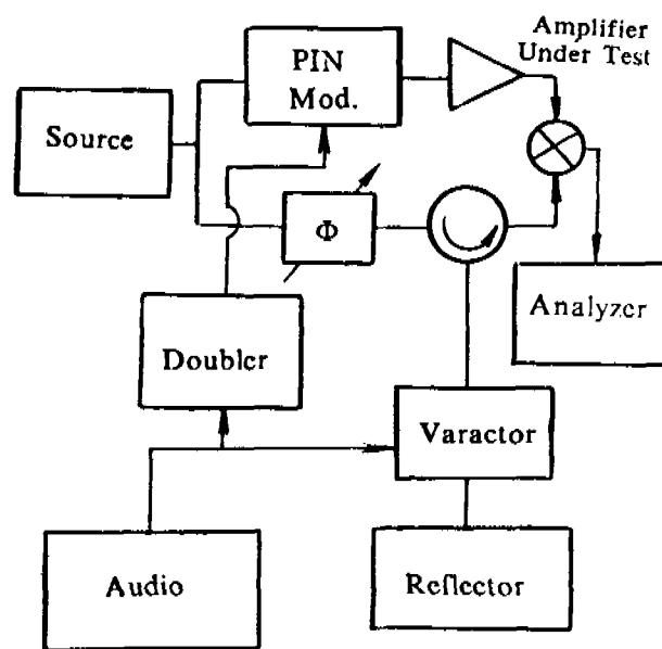
Figure 9. PM Calibration Block Diagram
