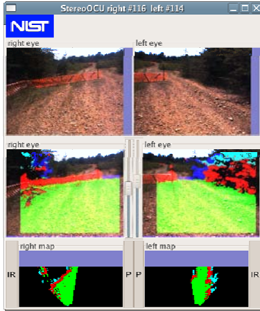
Figure 6. OCU display showing original images (top), results of obstacle detection (middle), and cost maps (bottom). Red represents obstacles, green is ground, and blue represents obstacles too far away to classify.
