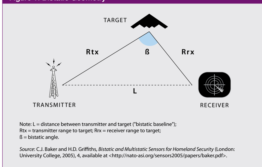
Figure 1. Bistatic Geometry
