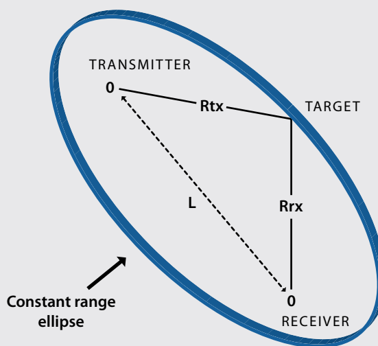
Figure 3. Bistatic Range
