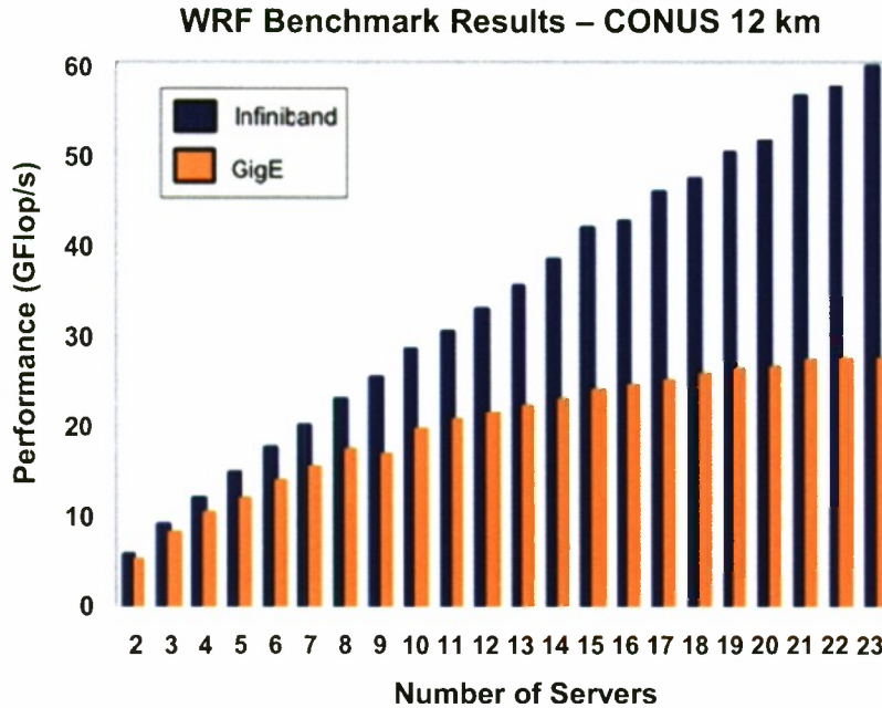
Figure 4. Scalability of Infiniband versus Gigabit Ethernet for weather model computations [3].
