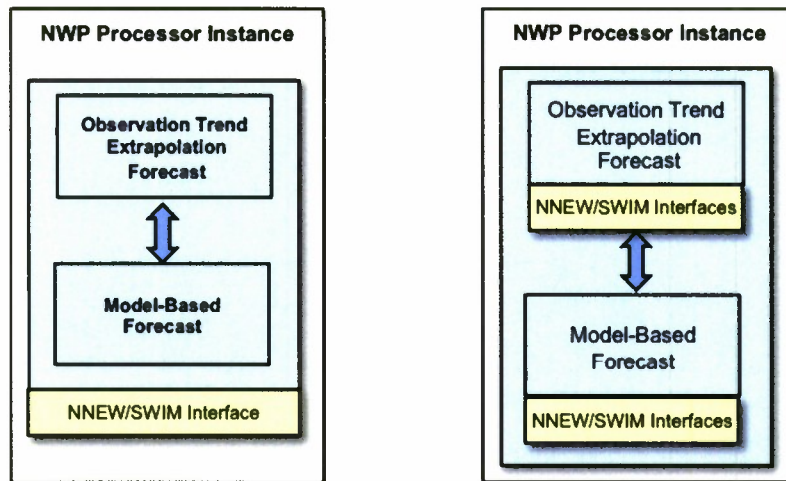
(a) Coarser-grained weather algorithm interface approach
