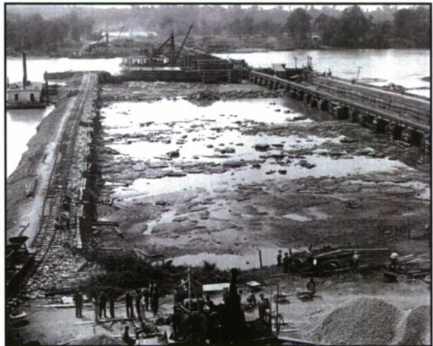
Plate 29. Wilson Lock and Dam, Tennessee River. View of interior of Cofferdam No. 1. Note that the river and upstream (left) arms of the cofferdam are of timber crib construction, while the downstream arm (right) is an Ohio River type box structure. 26 August 1919. RG77-RH, Box 169, Tennessee River Wilson L/D Cofferdam #1 Folder, NARA.
