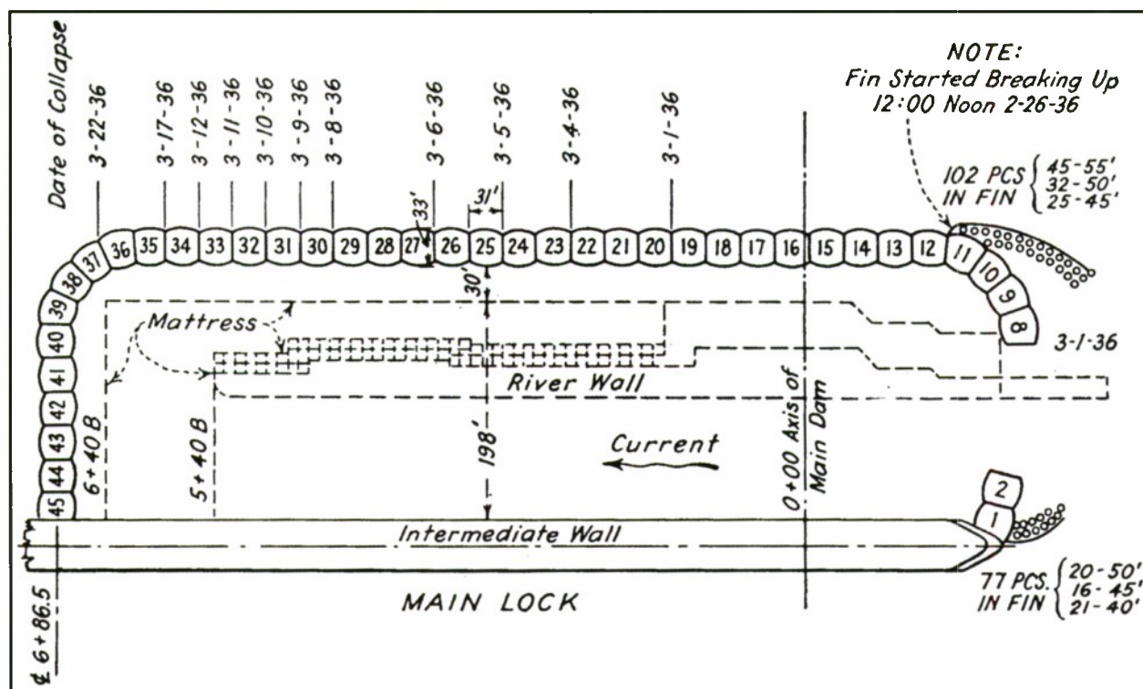
Figure 41. Mississippi River Lock and Dam No. 26. Plan of cofferdam for auxiliary lock. From White and Prentis, Cofferdams (1940).
