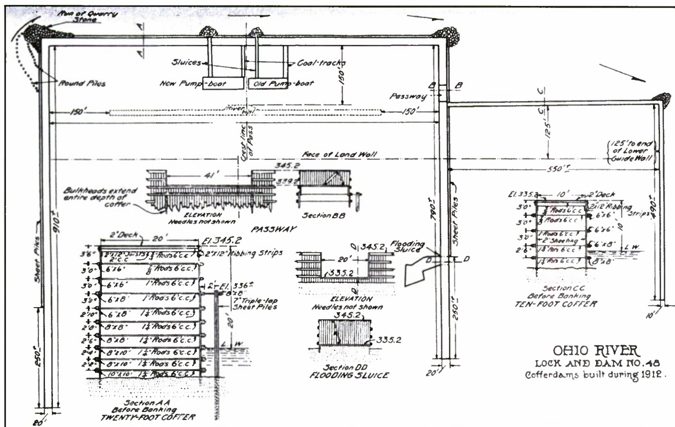
Figure 14. Ohio River Lock and Dam No. 48. Plan of 1912 cofferdam. From Oakes "Ohio River Dam No. 48" (1913).
