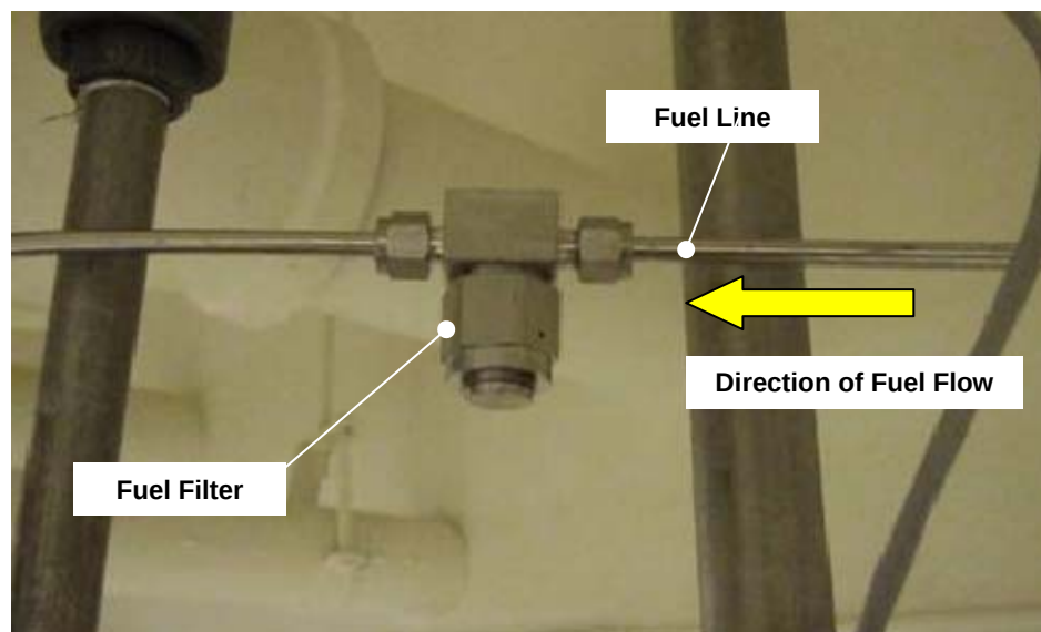
Figure 7. Fuel Filter (7 \mu\text{m} ) Installation
