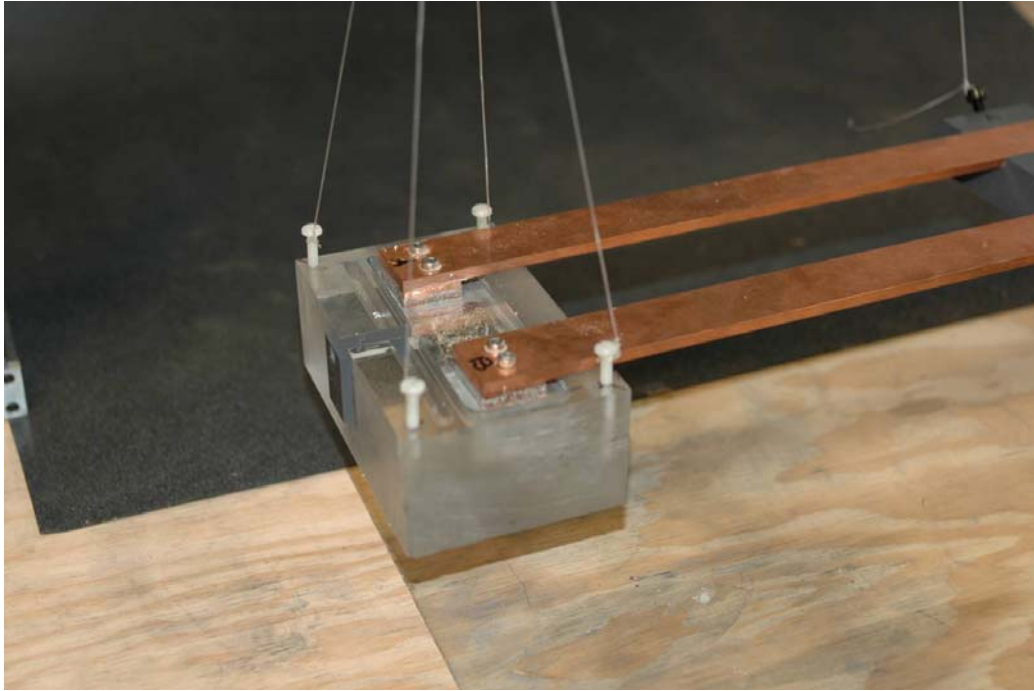
Figure 4. Rail/armature interface
