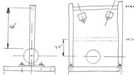
Figure 40. Potential Camera System for Angular Determination (After [53])
