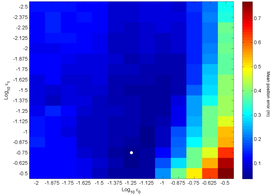
Figure SM3: Position error for different pairs (\varepsilon_0, \varepsilon_1) of parameters. The pair that produced the minimum position error (marked with a white 'o') was selected.
