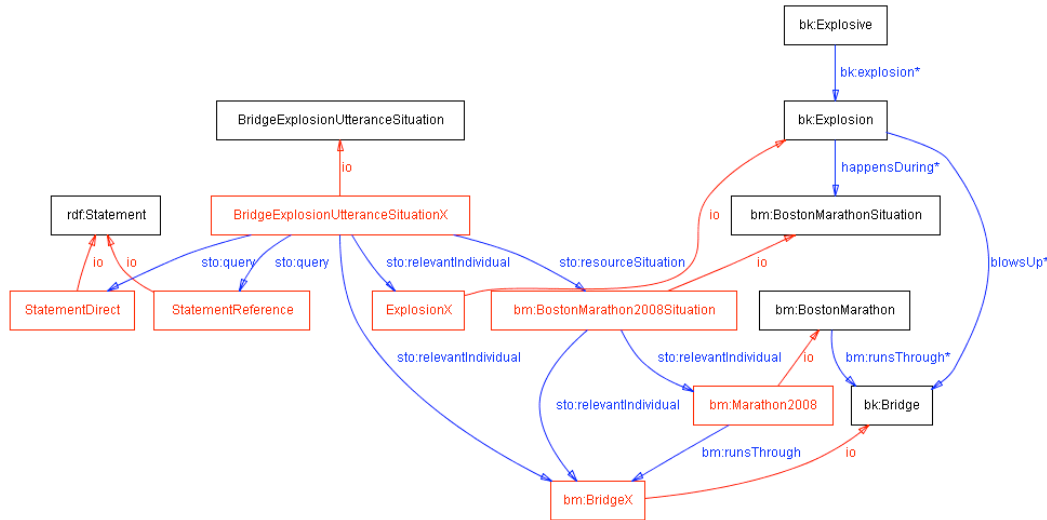
Figure 20 The [Bridge Explosion] Utterance Situation Ontology.
