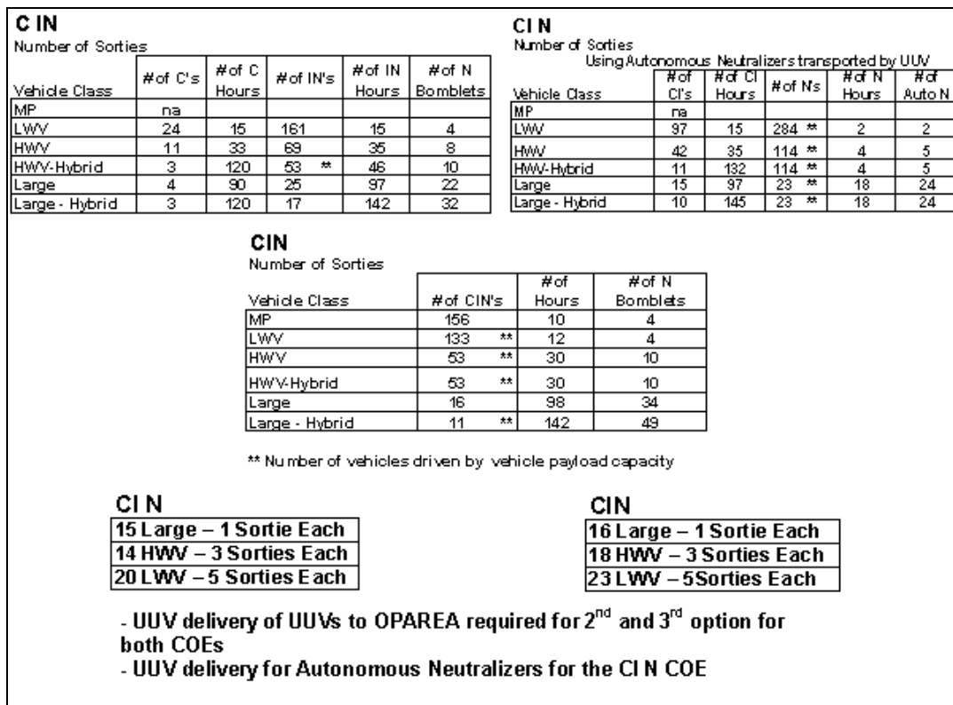
Figure 3-7. UUV System Options for MCM Missions
