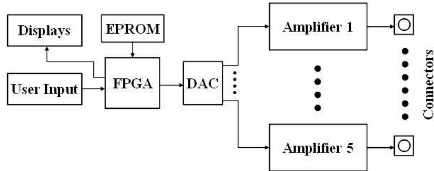
Figure 4.2: Architecture for the multichannel \pm 1.16 kV arbitrary waveform signal generator
