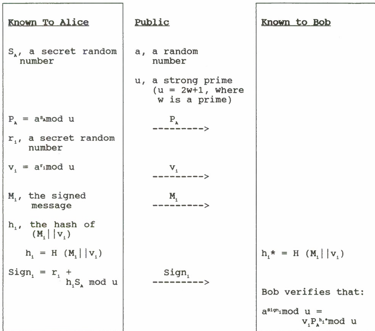
Figure 3: ElGamal Signature Algorithm: Alice sends a signature ( \text{Sign}_1 ) for message M_1 to Bob.
