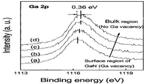
FIG. 25. XPS spectra of Ga 2p core level peaks for 400 °C annealed Pd/ Ir/Au contacts on p -GaN.
