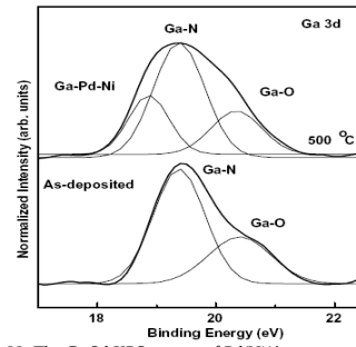
Fig. 22. The Ga 3d XPS spectra of Pd/Ni/Au contacts on p-GaN
