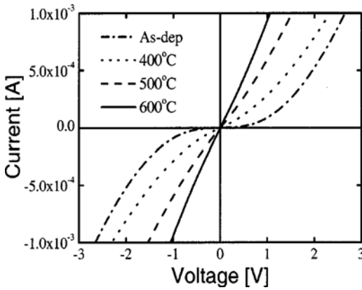
FIG. 14. I-V characteristics for the Pt/Pd/Au contacts on p -AlGaIn as a function of annealing temperature.
