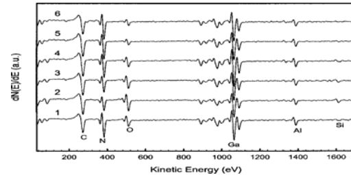
FIG. 13. AES surface scans of as-grown AlGaIn sample and those surface treated with SiCl 4 plasma at –300 V plasma bias voltage and then cleaned in NH 4 OH, HCl, BOE.
