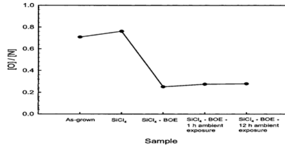
FIG. 11. Summary of ratio of O/N peak areas in the AlGaIn samples treated in BOE and exposed to air for various intervals of time.
