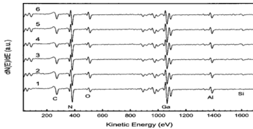
FIG. 12. AES surface scans of as-grown AlGaIn sample 1 and those surfaces treated with SiCl 4 plasma at different plasma bias voltages, –50 V, –100 V, –200 V, –300 V, and –400 V.
