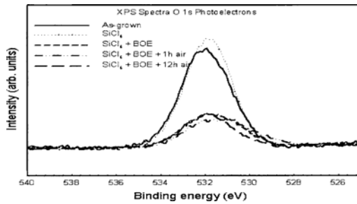
FIG. 10. XPS spectra of the O1s photoelectrons for the AlGaIn surface treated with BOE and then exposed to air for various intervals of time.
