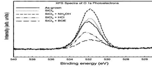
FIG. 8. XPS spectra of the \text{O}1s photoelectrons for the \text{AlGaIn} surface treated under several conditions
