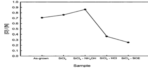
FIG. 9. Summary of ratio of \text{O/N} peak areas in the \text{AlGaIn} samples
