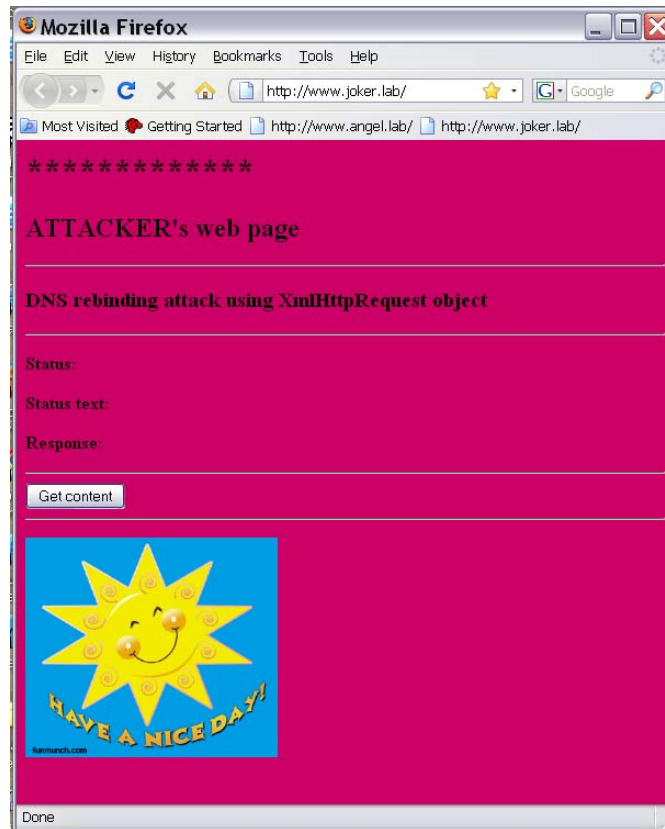
Figure 12. Victim client 2 retrieves attacker's home Web page
