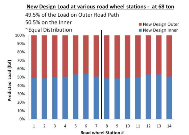
Figure 23: Expected nominal loading distribution
