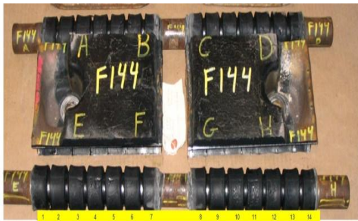
Figure 1A: Dissected T-158LL Track Block
