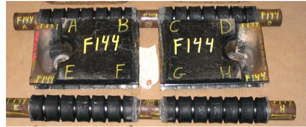
Figure 6: Example embrittlement and cracking of backer pad and bushing assembly M1
