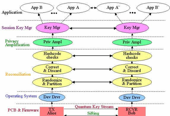
Figure 2. NIST QKD infrastructure protocol stack
