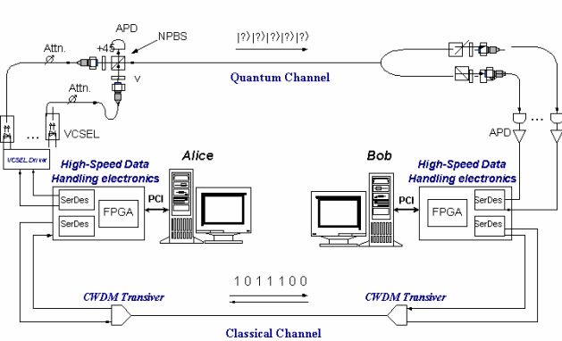
Figure 1. NIST QKD System Configuration
