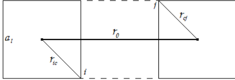
Fig. 2: The worst case \mathbf{r} and \mathbf{r}_0 , projected from the 3D box. Here, |\mathbf{r}_0| = 2a_l and i and j on at opposite corners of the box so that |\mathbf{r}| = |\mathbf{r}_{ic}| + |\mathbf{r}_{cj}| = a_l\sqrt{3} .
