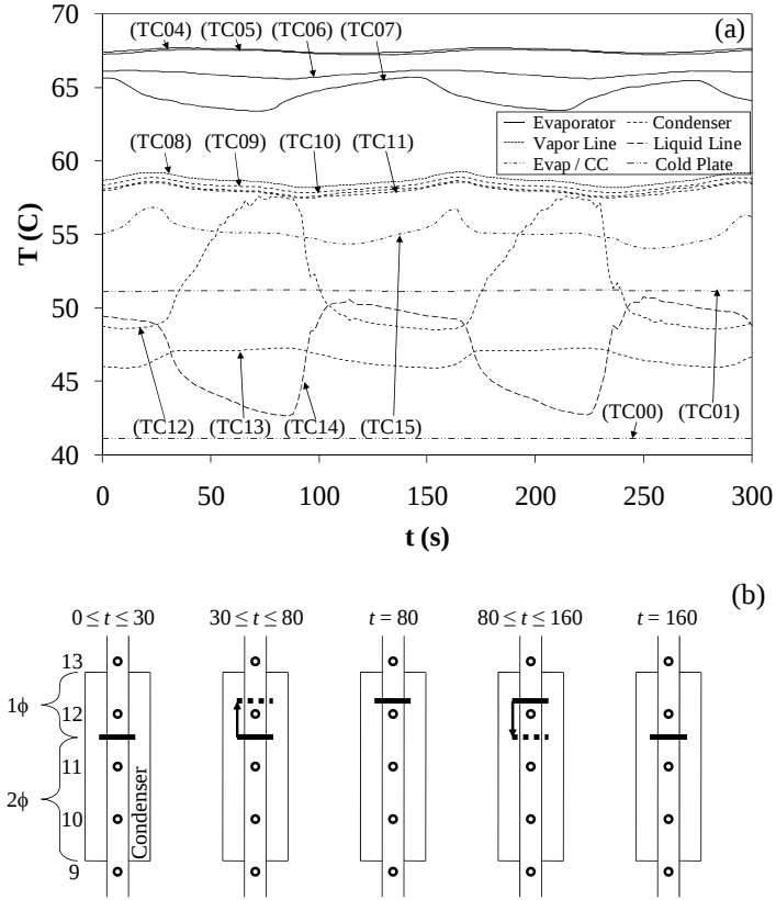
Figure 2.11. Transient temperature profiles of the stationary LHP for Q_{\text{in}} = 200 \text{ W} ( Q_{\text{cc}} = 0 \text{ W} , a_r = 0 \text{ g} , \dot{m}_{\text{cp}} = 0.0077 \text{ kg/s} , \bar{T}_{\text{cp}} = 46.1^{\circ}\text{C} , T_{\text{amb}} = 31.7^{\circ}\text{C} ): (a) Transient temperature profiles; (b) 2φ-1φ point oscillation in the condenser.
