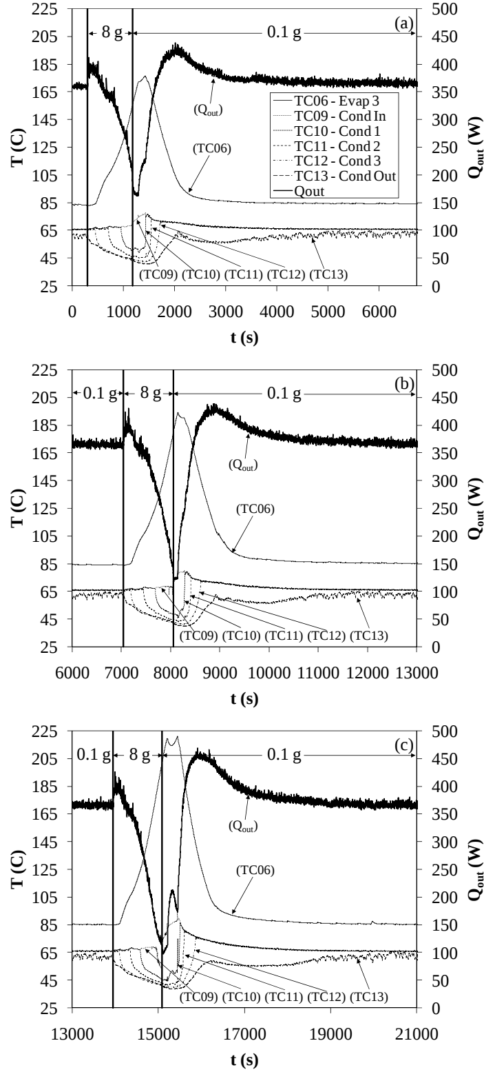
Figure 2.19. Transient temperature traces of the LHP at elevated acceleration showing dry-out behavior ( Q_{in} = 400 W, Q_{cc} = 0 W, \dot{m}_{cp} = 0.0077 kg/s, 37.2 \leq \bar{T}_{cp} \leq 59.7^{\circ}\text{C} , T_{amb} = 28.0^{\circ}\text{C} ): (a) T_{e,max} = 150^{\circ}\text{C} ; (b) T_{e,max} = 175^{\circ}\text{C} ; (c) T_{e,max} = 200^{\circ}\text{C} .
