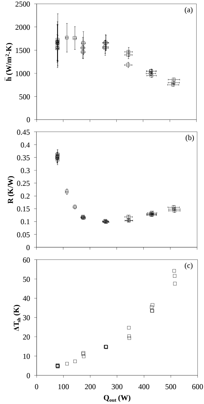
Figure 2.13. Steady state performance characteristics of the stationary LHP versus transported heat ( Q_{cc} = 0 W, a_r = 0 g, \dot{m}_{cp} = 0.0077 kg/s, 36.8 \leq \bar{T}_{cp} \leq 67.7^\circ C , 27.6 \leq T_{amb} \leq 38.7^\circ C ): (a) Evaporative heat transfer coefficient; (b) Thermal resistance; (c) Wall superheat
