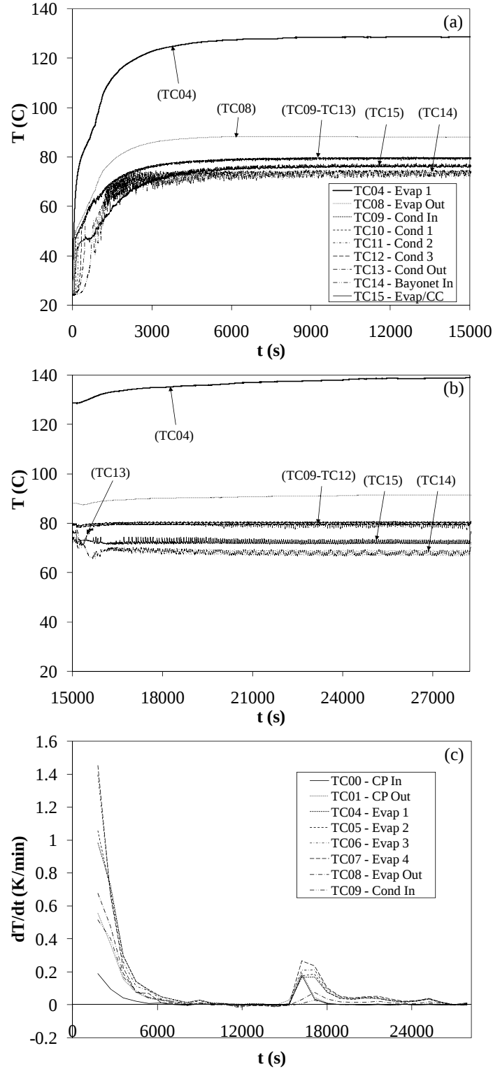
Figure 2.16. Transient temperature traces of the LHP at elevated acceleration ( Q_{in} = 600 W, Q_{cc} = 0 W, \dot{m}_{cp} = 0.0077 kg/s, 55.2 \leq \bar{T}_{cp} \leq 59.7^\circ\text{C} , 27.9 \leq T_{amb} \leq 30.1^\circ\text{C} ): (a) a_r = 0.1 g startup phase; (b) Transition to and steady state at a_r = 10.0 g; (c) Transient rate of change of temperatures.
