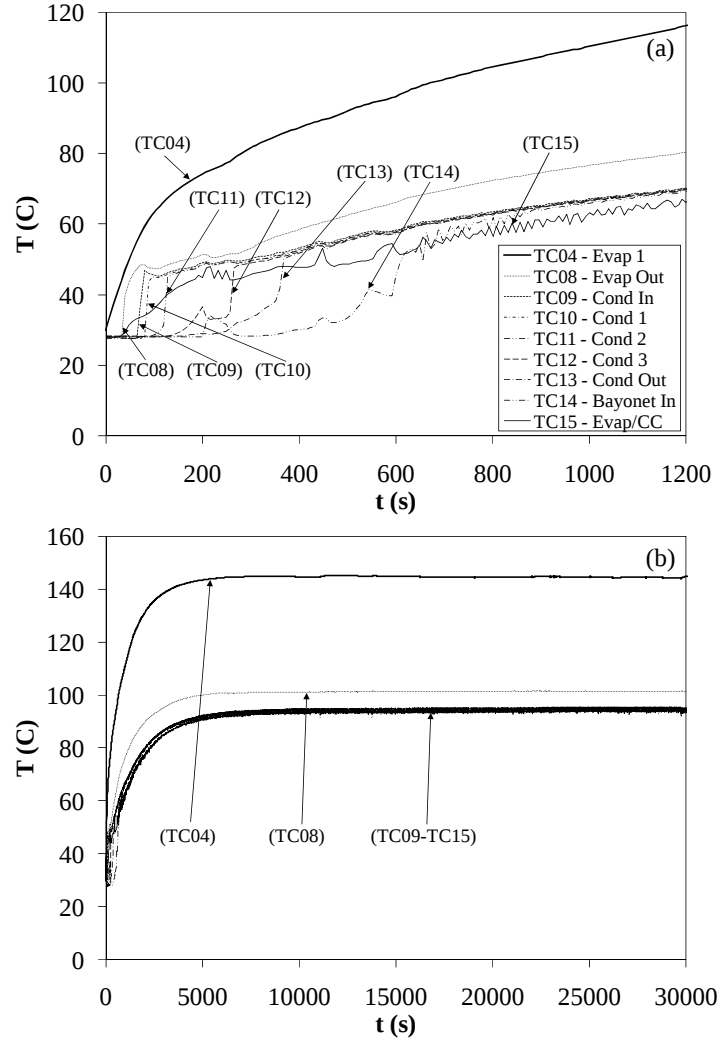
Figure 2.9. Transient startup of the stationary LHP ( Q_{\text{in}} = 600 W, Q_{\text{cc}} = 0 W, a_r = 0 g, \dot{m}_{\text{cp}} = 0.0077 kg/s, \bar{T}_{\text{cp}} = 67.7^\circ\text{C} , T_{\text{amb}} = 38.1^\circ\text{C} ): (a) Initial startup; (b) Complete startup until steady state.
