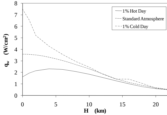
Figure 1.9. Average heat flux dissipated over the plate versus altitude for various atmospheric conditions ( T_w = 135^\circ\text{C} , L = 1.0 m, \text{Ma}_\infty = 0.98 ) (DOD, 1997; Anderson, 2000).
