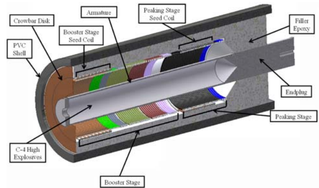
Fig. 5. Cutaway-view of dual stage helical flux compression generator, cf. Fig. 1 part B, with an explosive charge of \sim 410 \text{ g} of C-4. Overall length about 30 cm (12 in).
