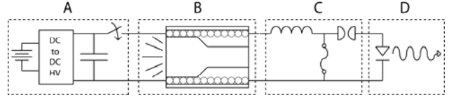
Fig. 1. Energy flow through sub-systems. Battery prime power and capacitor, HFCG, energy storage inductor with fuse opening switch and peaking gap, HPM source [4].
