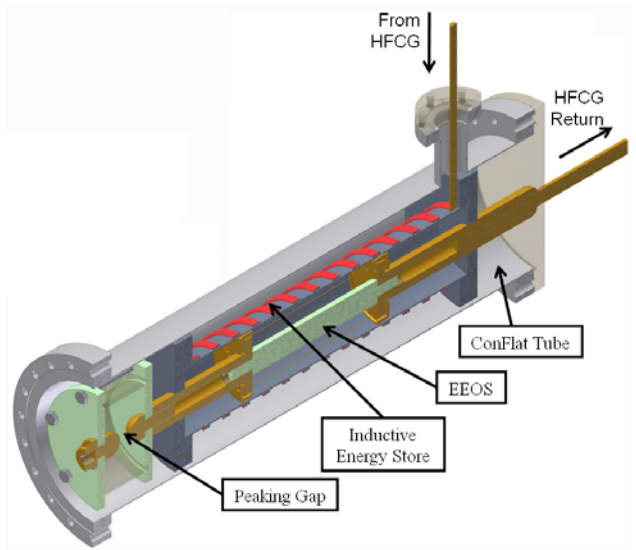
Fig. 8. Cutaway-view of Power Conditioning System with an \sim 2.25 \mu\text{H} energy storage inductance, cf. Fig. 1 part C. Overall length 24 cm ( \sim 2 \text{ ft} ).
