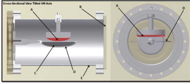
Fig. 10. Virtual cathode oscillator, cf. Fig. 1 part D. A-velvet cathode, B- microwave output window, C- anode mesh, D- anode holder, E- vacuum envelope.
