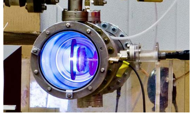
Fig. 12. Time integrated photograph of explosive-driven vircator [9].
