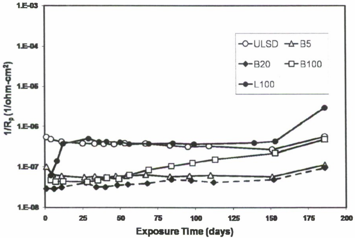
Figure 5. E_{corr} (V Hg/HgSO 4 ) and 1/R_p (instantaneous corrosion rate) trends for stainless steel S30403 exposed to each of the 5 fuel/water mixtures.
