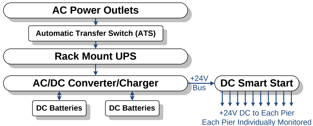
Figure 9. Dc power configuration.
