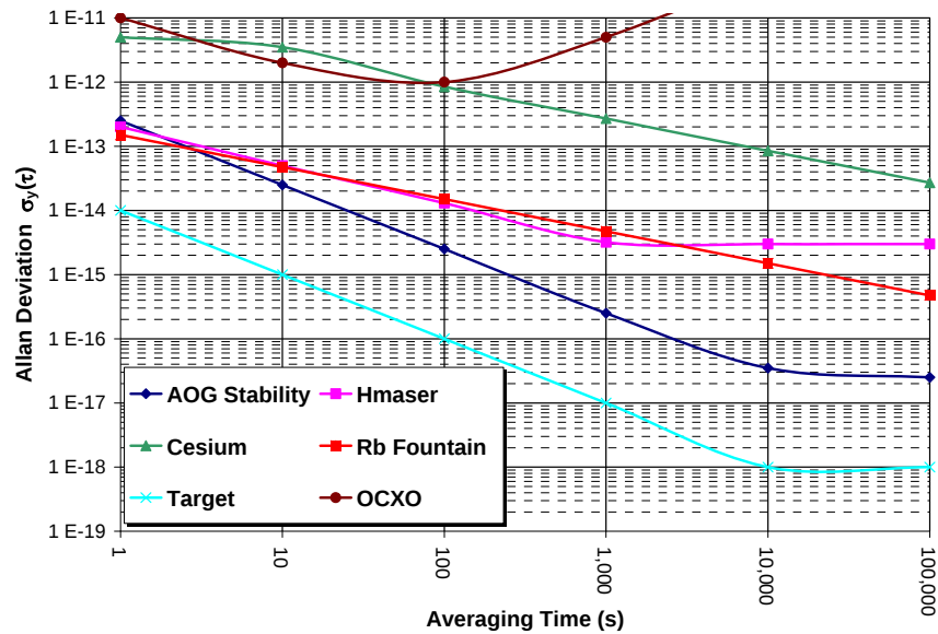
Figure 14. Allan deviation comparison graph.
