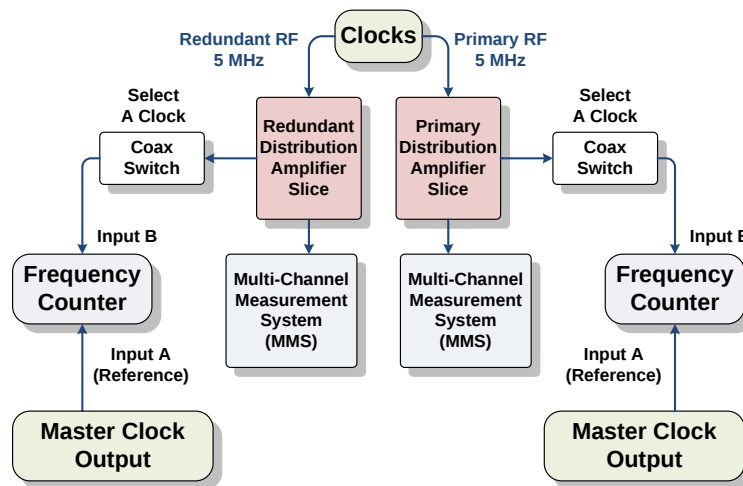
Figure 15. Measurement system configuration.
