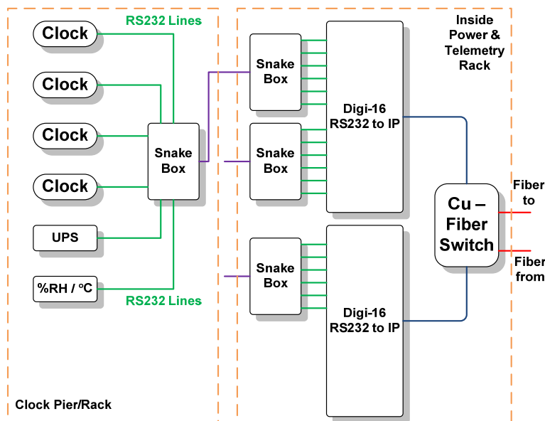
Figure 10. Telemetry configuration.
