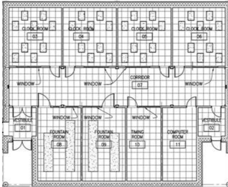
Figure 5. Pier layout.
