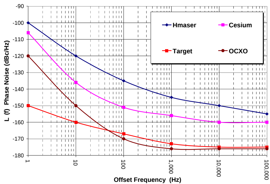
Figure 12. Phase noise comparison graph.
