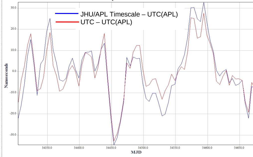
Fig. 5. Comparison of JHU/APL Timescale – UTC (APL) and UTC – UTC (APL), showing high correlation of 0.939, slope and drift removed from both plots.
