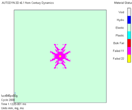
Figure 4: Simulated impact at 846 m/s
