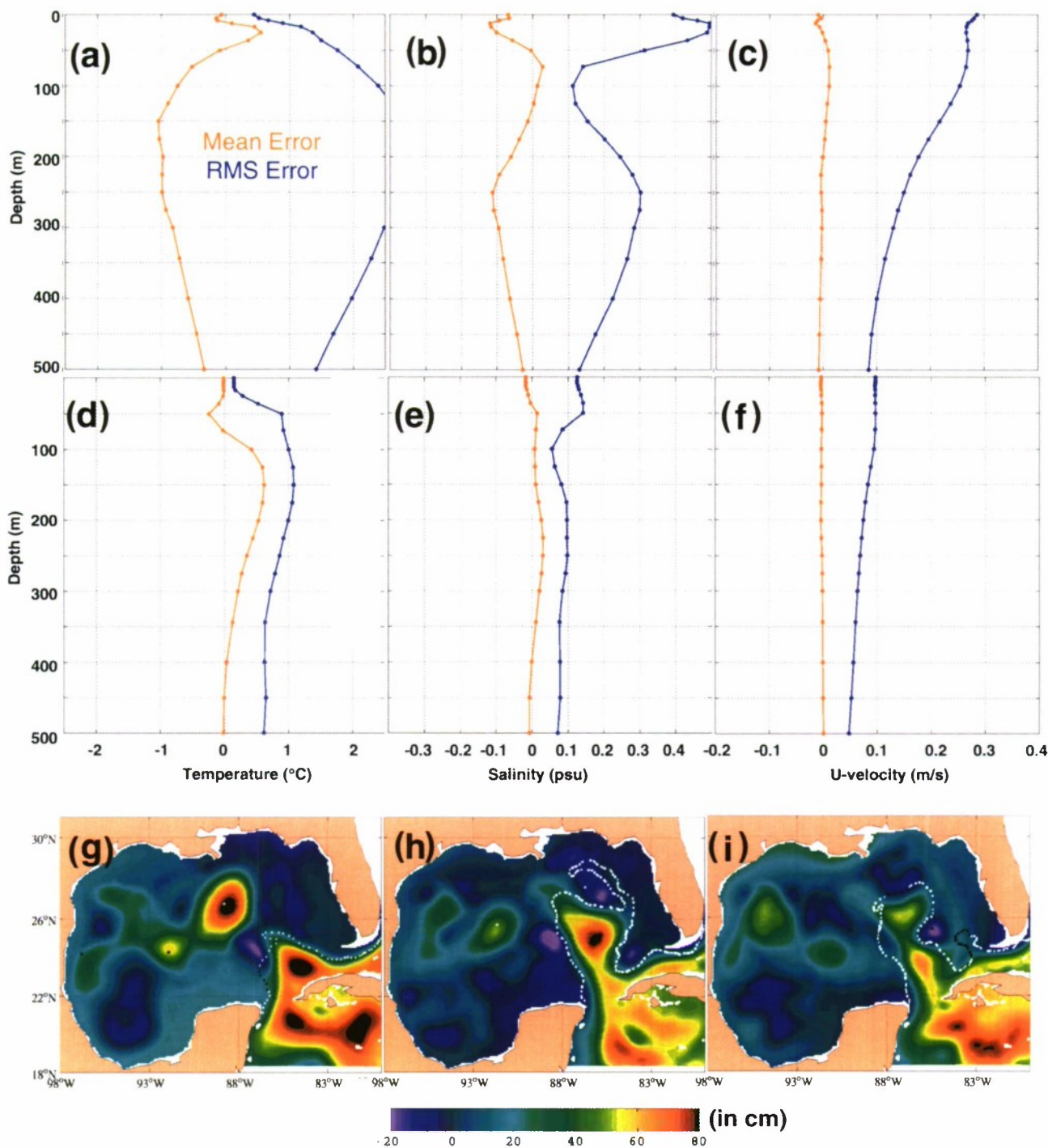
Plate 6. (a-f) Verification of SST and altimeter track SSH assimilation in 1/12° Gulf of Mexico HYCOM using NCODA and data simulated by the model during a different time period as sampled at observed SST and altimeter track locations during that time. Mean error (red) and rms error (blue) versus depth to 500 m for (a, d) temperature, (b, e) salinity, and (c, f) zonal component of velocity at the beginning of the assimilation period on August 29, 1999, and 50 days later on October 18, 1999. (g-i) Results of assimilating real SST, temperature profile, and altimeter track data into 1/12° Gulf of Mexico HYCOM and verification against operational NAVOCEANO frontal analyses of satellite infrared imagery overlaid on HYCOM SSH fields for (g) October 18, 1999, (h) March 6, 2000, and (i) May 4, 2000. Black dotted segments of the frontal analyses are based on infrared imagery more than 4 days old.
