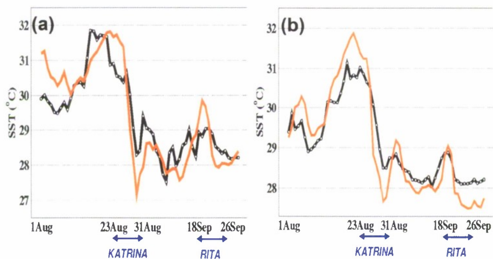
Plate 5. Daily observed buoy SST (black lines) versus 1/12^\circ global HYCOM (red lines) using three-hourly FNMOC NOGAPS wind and thermal forcing. The time series span from August 1 to September 30, 2005 and cover the passage of Hurricanes Katrina and Rita at (a) NDBC buoy 42040 south of Mobile Bay and (b) buoy 42036 southeast of Pensacola, FL.
