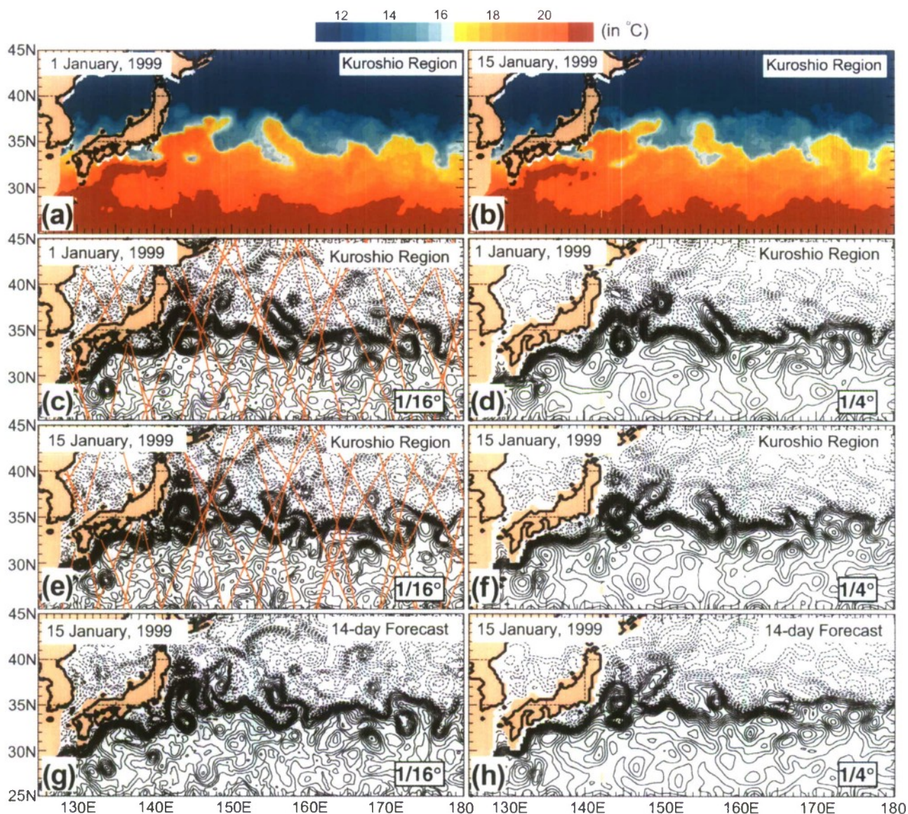
Plate 1. Kuroshio region (a, b) NAVOCEANO operational 1/8° MODAS SST analyses for (a) January 1, 1999 and (h) January 15, 1999 with the color bar (0.5°C interval) designed to highlight the Kuroshio pathway, (c-f) SSH analyses (5-cm interval) with assimilation of altimeter track data from TOPEX/Poseidon and ERS-2 using the model forecast as the first guess from (c, e) 1/16° Pacific NLOM and (d, f) 1/4° global NLOM for (c, d) January 1, 1999 and (e, f) January 15, 1999. The altimeter tracks assimilated on the date given (using a 3-day data window) are overlaid in red on (c, e). (g, h) The 14-day forecast SSH from (g) 1/16° Pacific NLOM and (h) 1/4° global NLOM. Adapted from Hurlburt et al. [2000].
