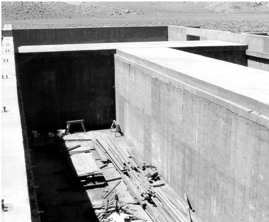
Figure 10. Portion of transfer aisle walls.
