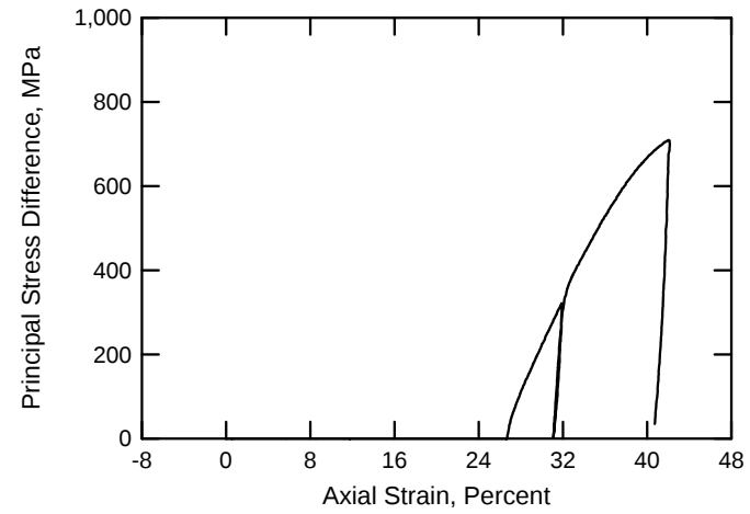
Type N Mortar Test No. 53
