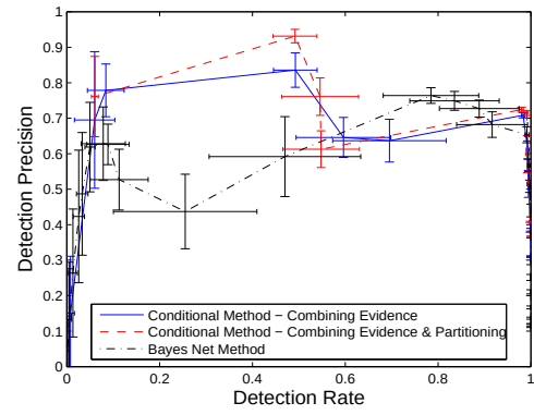
(b) Mailbomb
