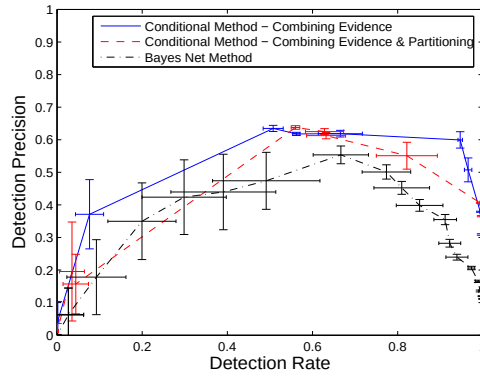
(c) Snmpguess
